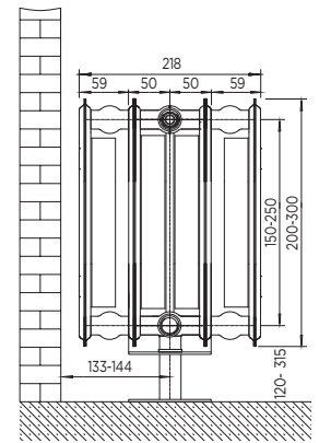
QS Quadruple Panel Quadruple Convactor
